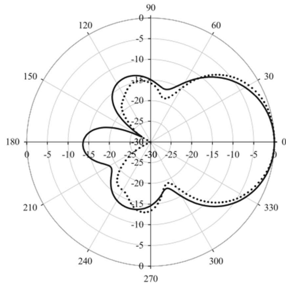
Fig. 2 (a) Measured and Simulation radiation pattern of the proposed antenna at 2.4 GHz in (a) XZ plane and (b) YZ planes. We measured and Simulated the radiation pattern of the proposed antenna at 2.45 GHz in (c) XZ plane and (d) YZ planes. We measured and Simulated the
