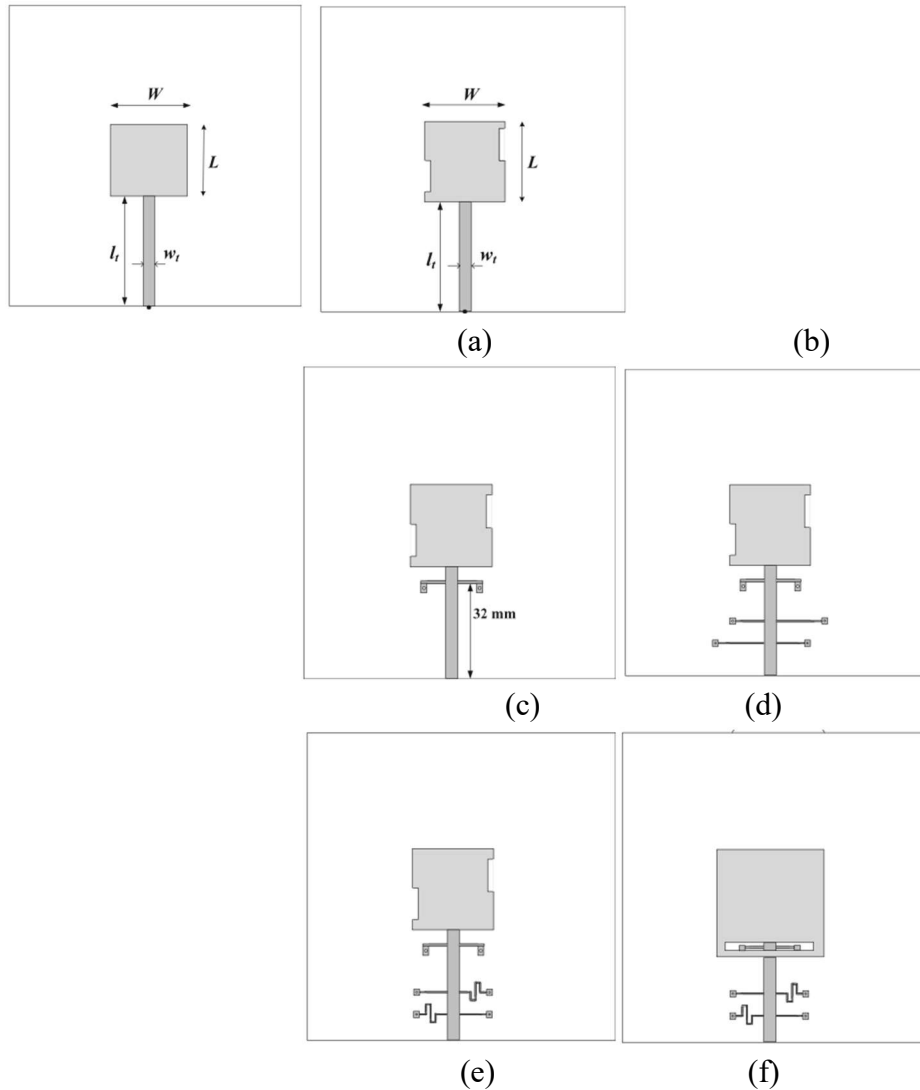
Fig. 1 (a) Basic patch antenna with dimensions ( L = W = 28\text{mm} , l_f = 36\text{mm} and w_f = 2.8\text{mm} ), (b) Improved patch antenna with an asymmetrical cut at left and right edges, (c) Improved patch antenna with shunt inductor at 32mm above from feed point, (d) Improved patch antenna with microstrip resonators, (e) Improved patch antenna with microstrip symmetrical resonators, and (f) Improved patch antenna with parasitic patch and slot[14,15].
